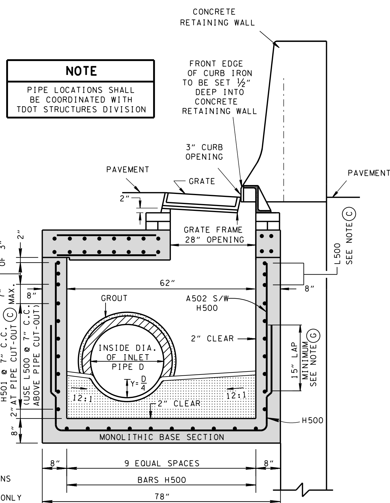
SECTION B-B
